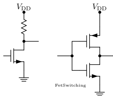
Figure 2: Simple FET Switch and a CMOS Inverter
