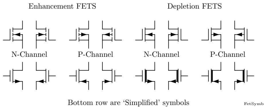
Figure 1: Symbols of MOSFETS
